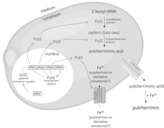
Figure 3. The metabolic pathway of pulcherriminic acid (Source: Puyo et al., 2023)
