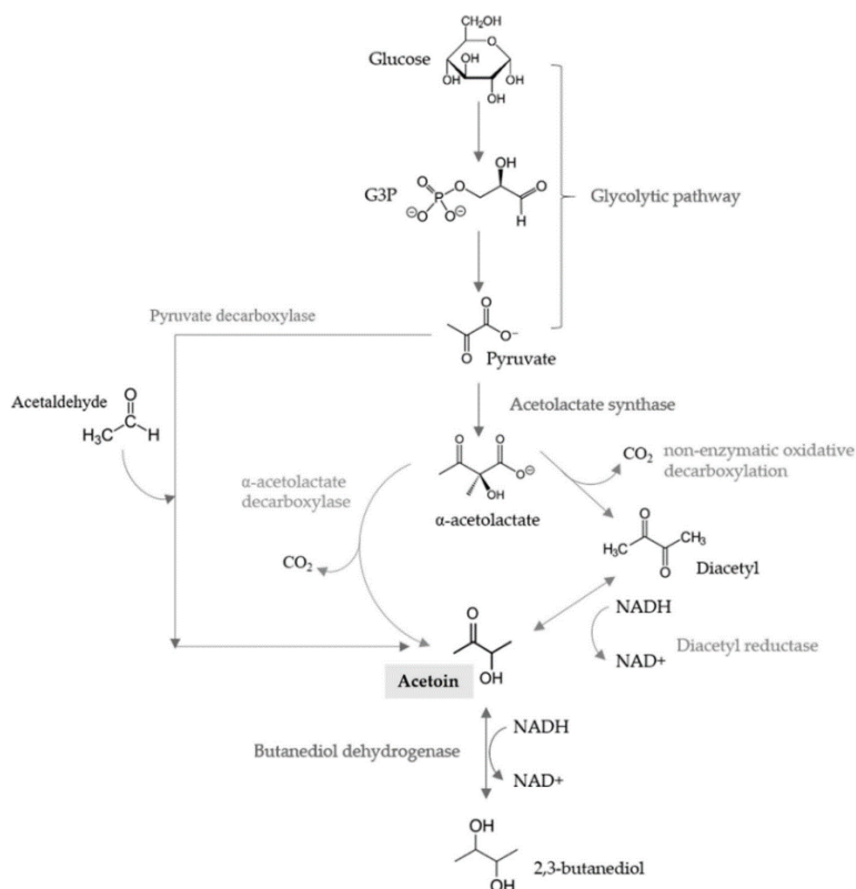
Figure 2. Pathway of yeast acetoin biosynthesis (Source: Romano & Suzzi, 1996)
