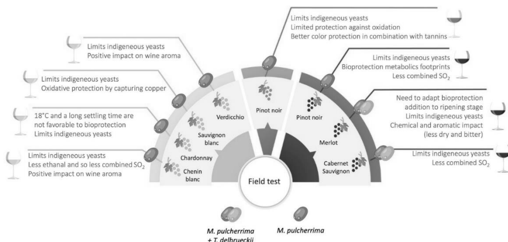
Figure 4. The applied field of use of M. pulcherrima (Source: Puyo et al., 2023)
